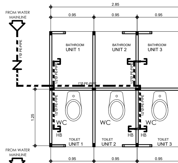
2 P-02 DUPEX 3-SET T&B PLUMBING LAYOUT SCALE 1:50 M
