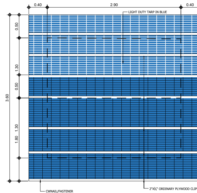
2 A-06 DUPLEX 3-SET T&B ROOF PLAN SCALE 1:100 M
