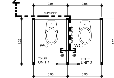
6 P-02 SINGLE 2-SET TOILET PLUMBING LAYOUT SCALE 1:50 M
