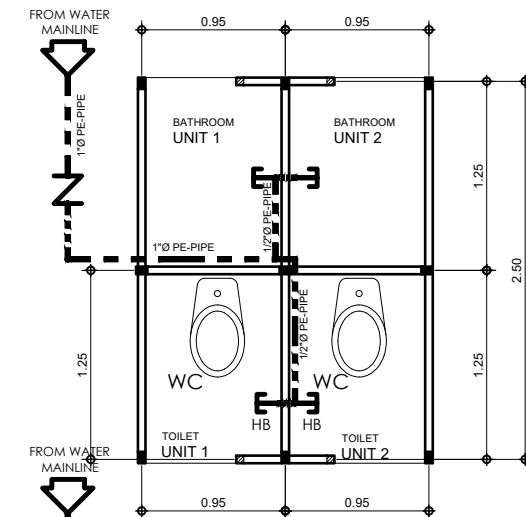
3 P-02 DUPEX 2-SET T&B PLUMBING LAYOUT SCALE 1:50 M
