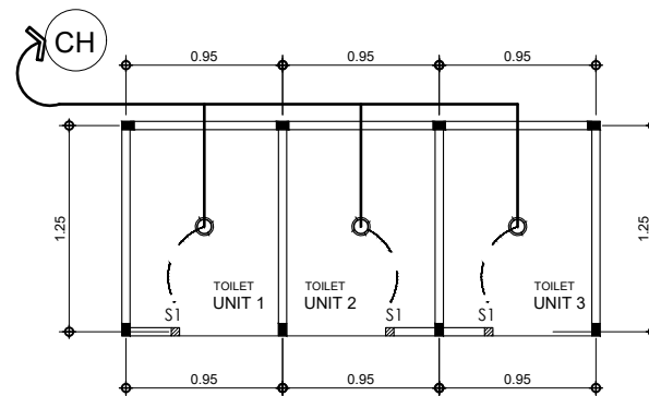
8 E-01 SINGLE 3-SET TOILET ELECTRICAL LIGHTING LAYOUT SCALE 1:50 M
