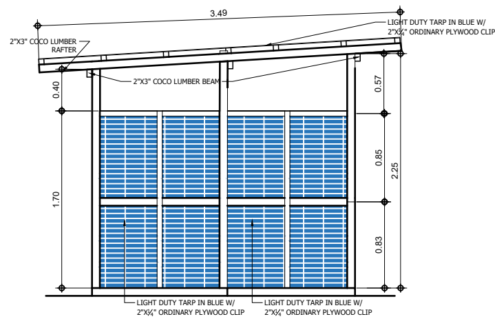
4 A-07 SCALE 50 M SIDE ELEVATION FOR DUPLEX T&B
