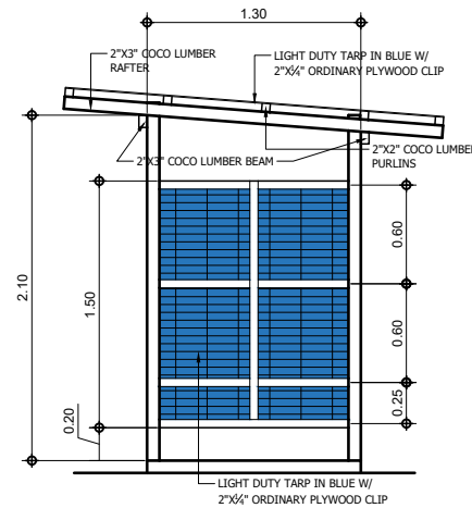
5 A-07 SCALE 50 M SIDE ELEVATION FOR SINGLE T&B
