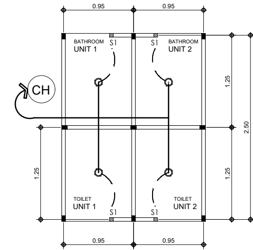
3 E-01 DUPLEX 2-SET T&B ELECTRICAL LIGHTING LAYOUT SCALE 1:50 M
