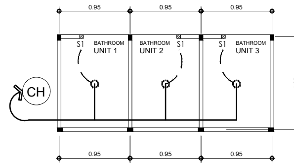
5 E-01 SINGLE 3-SET BATH ELECTRICAL LIGHTING LAYOUT SCALE 1:50 M
