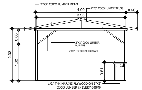
8 A-07 SCALE 1:100 M MAKESHIFT KITCHEN FRONT ELEVATION
