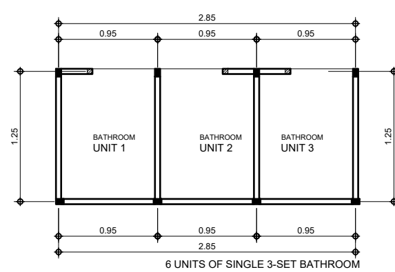
6 A-05 SCALE 1:100 M SINGLE 3-SET BATHROOM FLOOR PLAN
