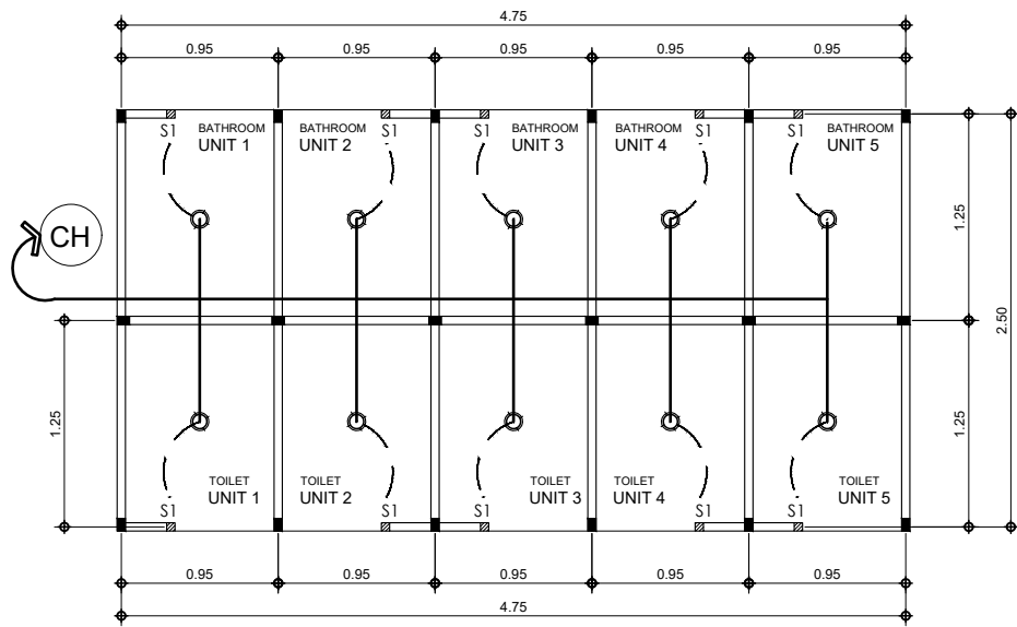
1 E-01 DUPLEX 5-SET T&B ELECTRICAL LIGHTING LAYOUT SCALE 1:50 M
