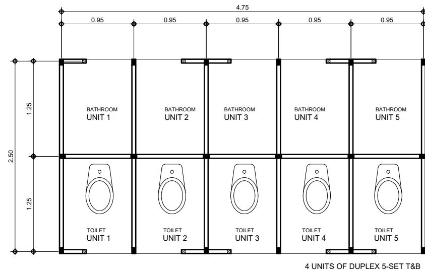
1 A-05 SCALE 1:100 M DUPLEX 5-SET T&B FLOOR PLAN
