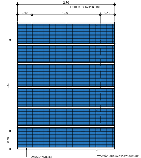
3 A-06 DUPLEX 3-SET T&B ROOF PLAN SCALE 1:100 M
