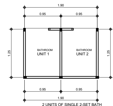
9 A-05 SCALE 1:100 M SINGLE 2-SET BATHROOM FLOOR PLAN
