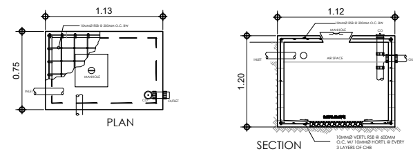
8 P-01 SEPTIC VAULT DETAIL SCALE 1:50 M
