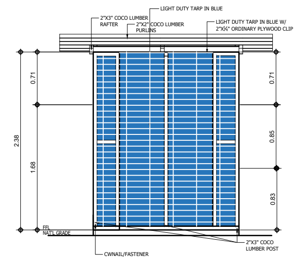
6 A-06 DUPLEX 2-SET T&B FRONT ELEVATION SCALE 1:100 M
