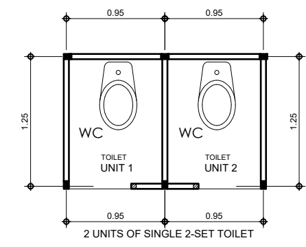
8 A-05 SCALE 1:100 M SINGLE 2-SET TOILET FLOOR PLAN
