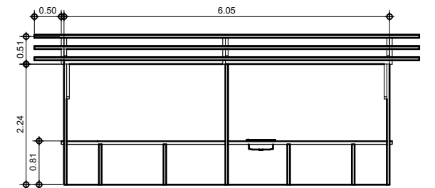
6 A-07 SCALE 1:100 M MAKESHIFT KITCHEN FRONT ELEVATION
