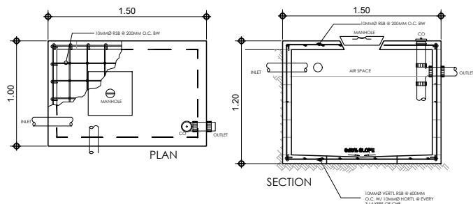
7 P-01 SEPTIC VAULT DETAIL SCALE 1:50 M
