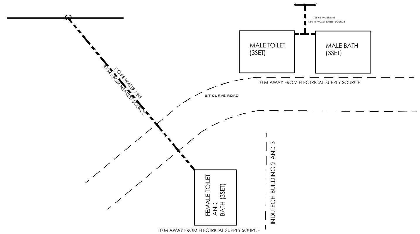
4 LOCATION MAP 17 A-04 SCALE 100 M
