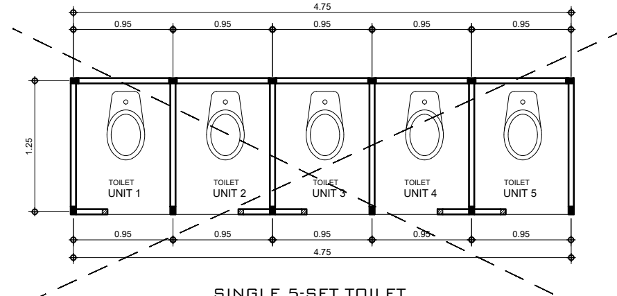
2 A-05 SCALE 1:100 M SINGLE 5-SET TOILET FLOOR PLAN
