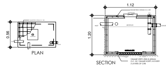
9 P-01 SEPTIC VAULT DETAIL SCALE 1:50 M
