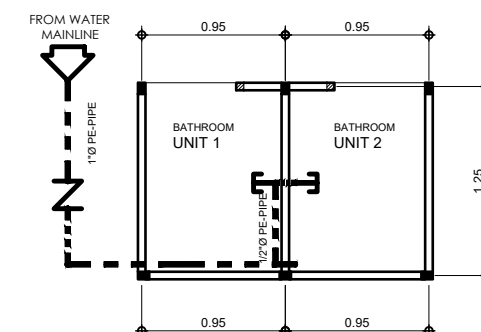
9 P-02 SINGLE 2-SET BATH PLUMBING LAYOUT SCALE 1:50 M
