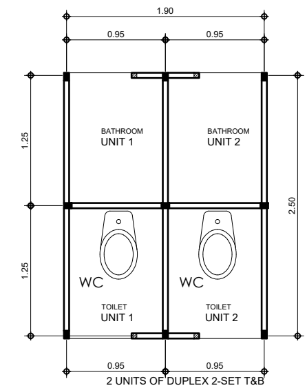
7 A-05 SCALE 1:100 M DUPLEX 2-SET T&B FLOOR PLAN
