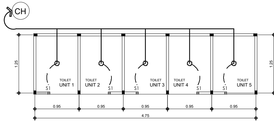
4 E-01 SINGLE 5-SET TOILET ELECTRICAL LIGHTING LAYOUT SCALE 1:50 M
