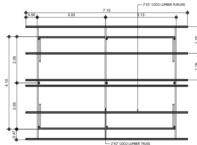
7 A-07 SCALE 1:100 M MAKESHIFT KITCHEN ROOF PLAN
