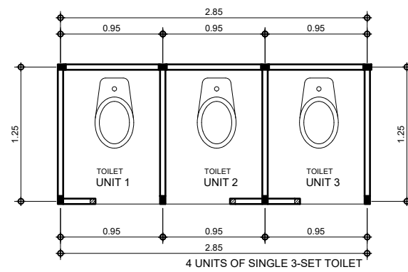
5 A-05 SCALE 1:100 M SINGLE 3-SET TOILET FLOOR PLAN
