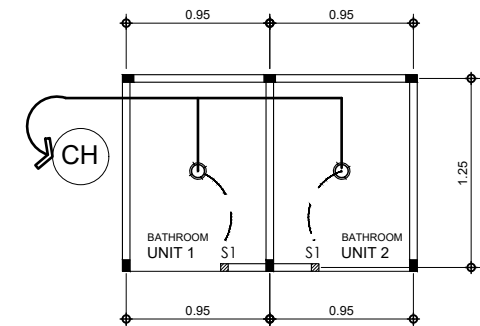
9 E-01 SINGLE 2-SET TOILET ELECTRICAL LIGHTING LAYOUT SCALE 1:50 M
