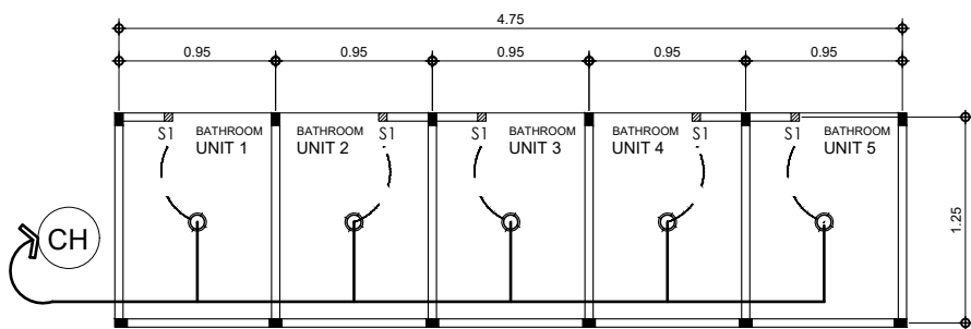
4 E-01 SINGLE 5-SET TOILET ELECTRICAL LIGHTING LAYOUT SCALE 1:50 M
