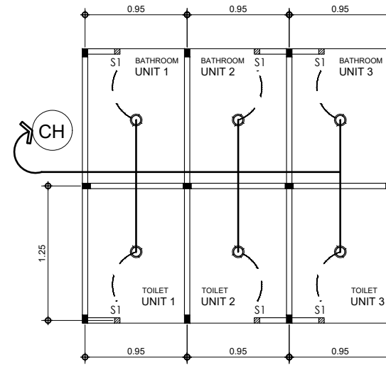
2 E-01 DUPLEX 3-SET T&B ELECTRICAL LIGHTING LAYOUT SCALE 1:50 M
