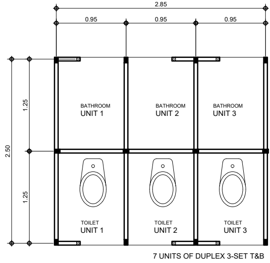
4 A-05 SCALE 1:100 M DUPLEX 3-SET T&B FLOOR PLAN
