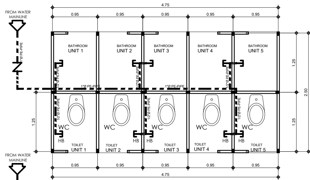
1 P-02 DUPEX 5-SET T&B PLUMBING LAYOUT SCALE 1:50 M
