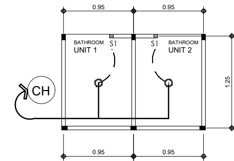
6 E-01 SINGLE 2-SET BATH ELECTRICAL LIGHTING LAYOUT SCALE 1:50 M
