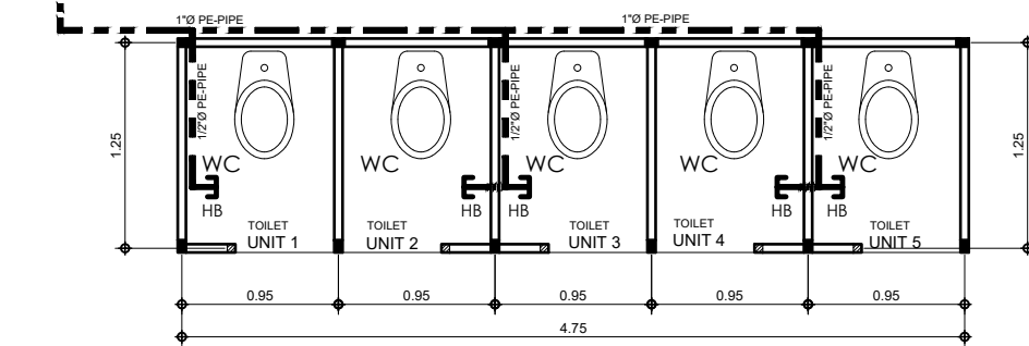
4 P-02 SINGLE 5-SET TOILET PLUMBING LAYOUT SCALE 1:50 M
