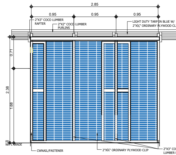
5 A-06 DUPLEX 3-SET T&B FRONT ELEVATION SCALE 1:100 M
