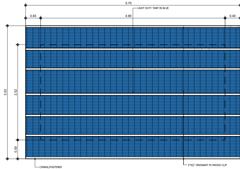
1 A-06 DUPLEX 5-SET T&B ROOF PLAN SCALE 1:100 M
