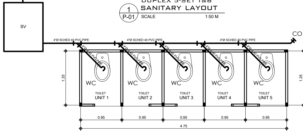
4 P-01 SINGLE 5-SET TOILET SANITARY LAYOUT SCALE 1:50 M
