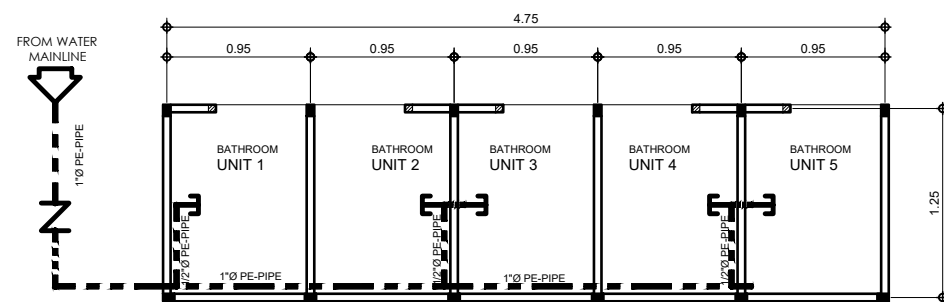
7 P-02 SINGLE 5-SET BATH PLUMBING LAYOUT SCALE 1:50 M
