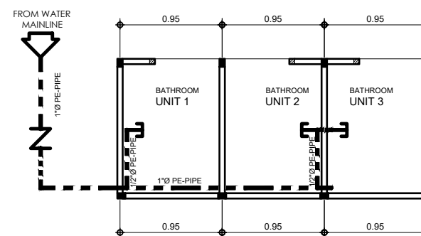
8 P-02 SINGLE 3-SET BATH PLUMBING LAYOUT SCALE 1:50 M
