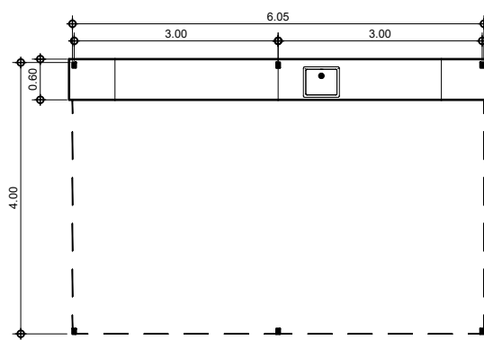
7 A-07 SCALE 1:100 M MAKESHIFT KITCHEN FLOOR PLAN
