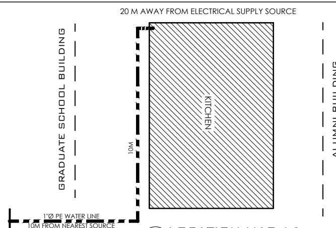
6 LOCATION MAP 16 A-03 SCALE 100 M
