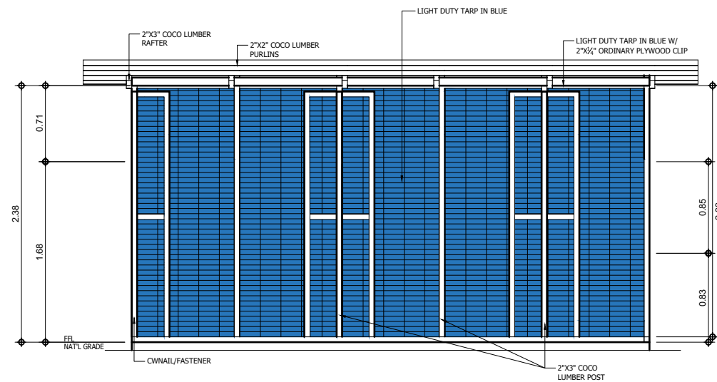
4 A-06 DUPLEX 5-SET T&B FRONT ELEVATION SCALE 1:100 M
