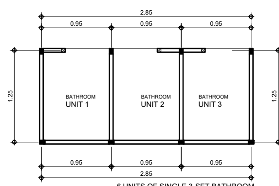
6 A-05 SCALE 1:100 M SINGLE 3-SET BATHROOM FLOOR PLAN
